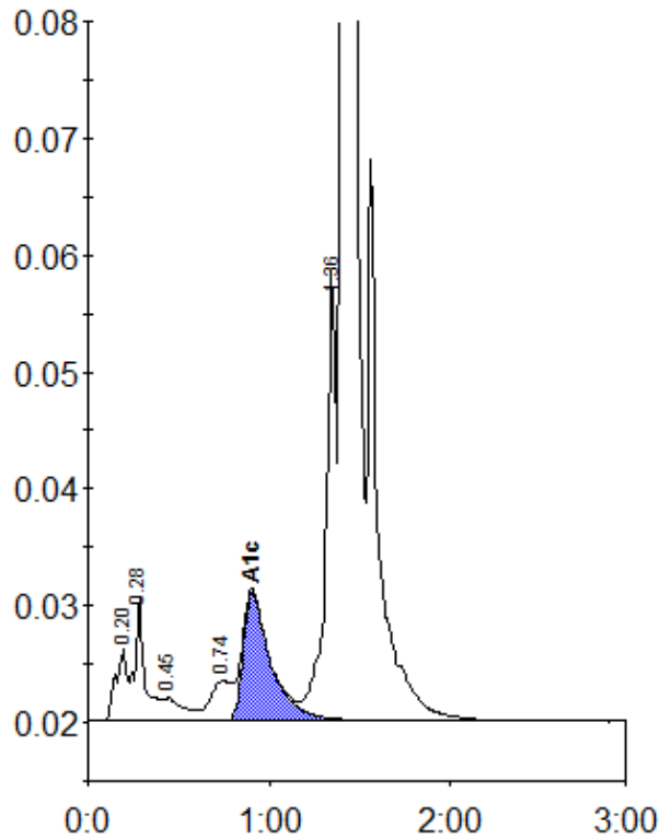
Peak table - ID: 10612854
